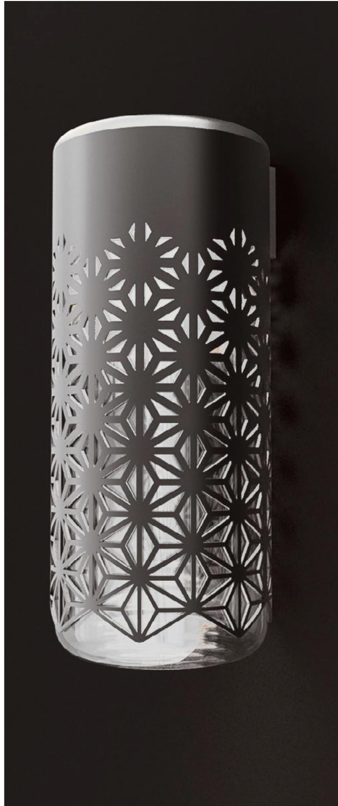
C18AL-0001-Do3Roo D.15 cm • H. 35 cm • P. 15.7 cm 1 x LED 9,1W 350mA - 2700, 3000, 3500, 4000, 5000, 5700, CRI90 options - customizable with dim to warm source - driver included - eBLUE Bluetooth + Casambi App for iOS and Android available optional. Customization: light / light control / finishing / dimension / cluster
